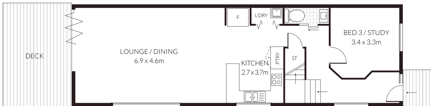
GROUND FLOOR
