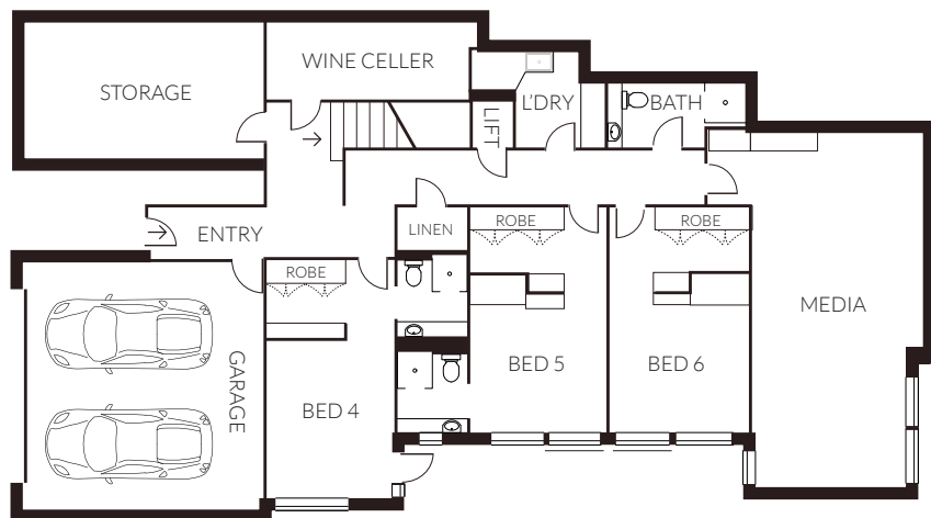
LOWER LEVEL
