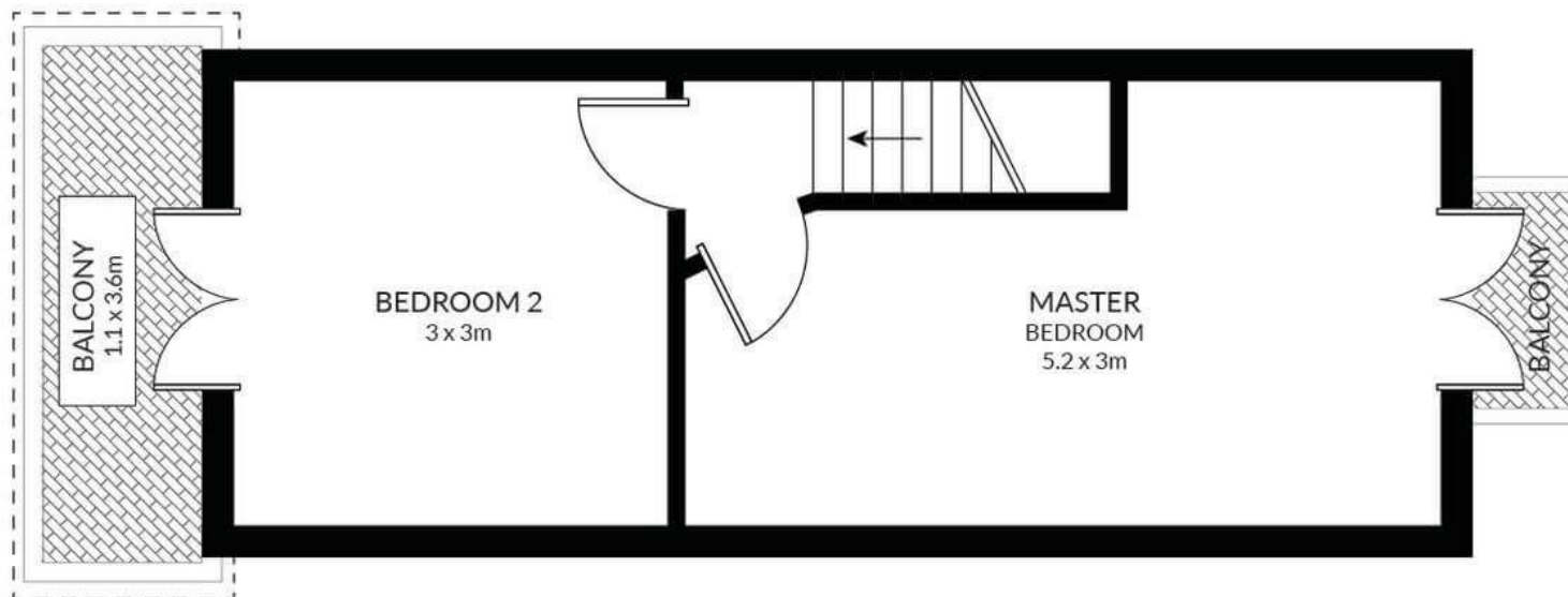
FIRST FLOOR
