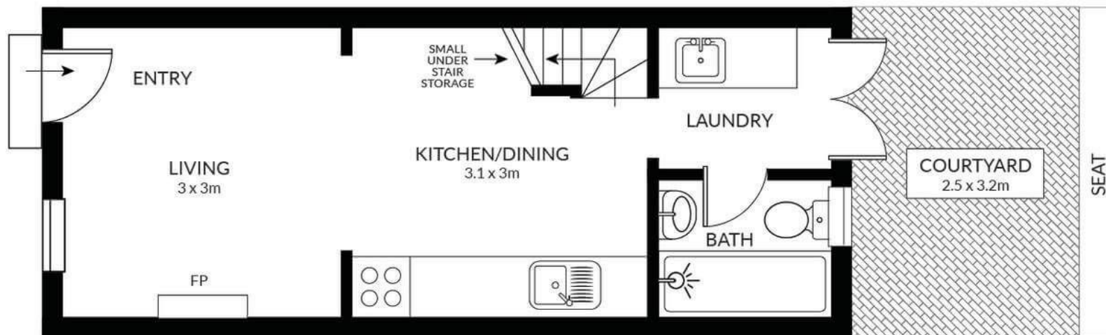
GROUND FLOOR
