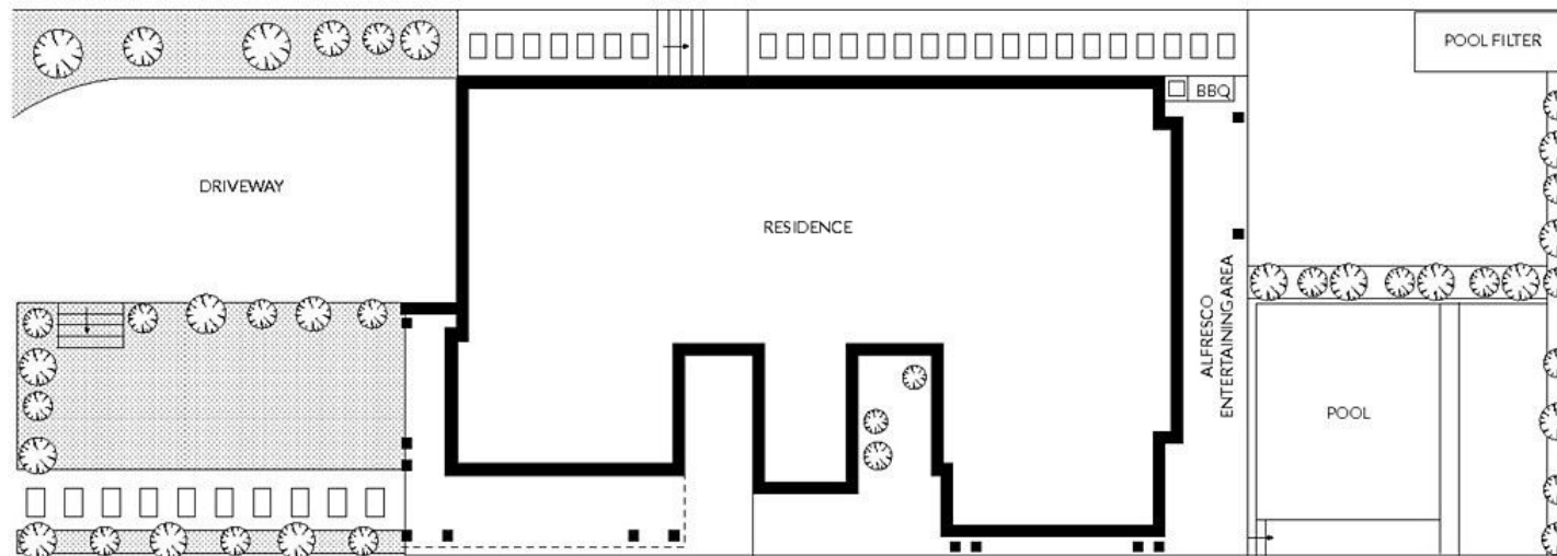
SITE PLAN
